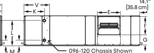
Right View Left Return Straight Discharge
