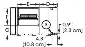
Back View Left Return Back Discharge
